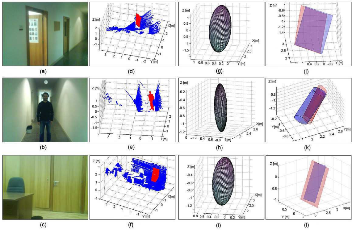
Fig. 6: Real data for testing the shape retrieval algorithms: a-c) Test sites for the real experiments; d-f) Real observations from an Hokuyo laser sensor (3-dimensions); g-i) Gaussian functions associated to the novelty; and j-l) Shapes generated by the algorithms (red: method based on Mathematical space of Gaussian mixture; blue: method based on Euclidean space).
